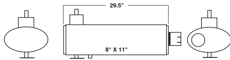
MODEL: CAT D8K 6N5437
