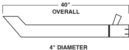
MODEL: CAT D6H STACK 7W5838
