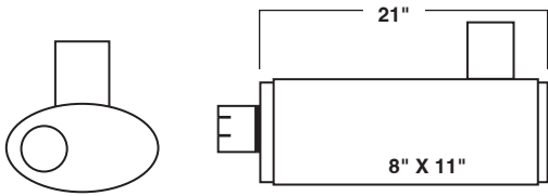
(ALSO ON PAGE OR10) MODEL: CAT 215 EXCAVATOR 6C0482
